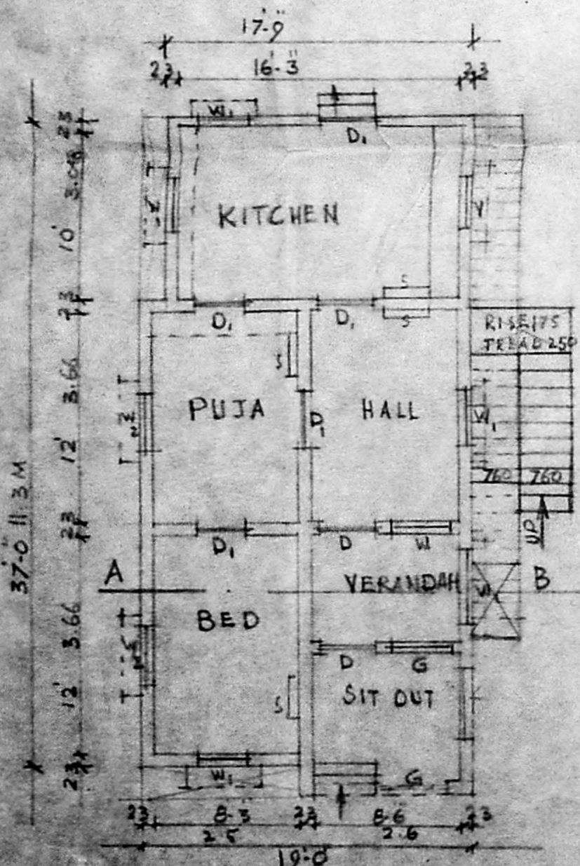
EXG. PLAN OF GROUND FLOOR.
