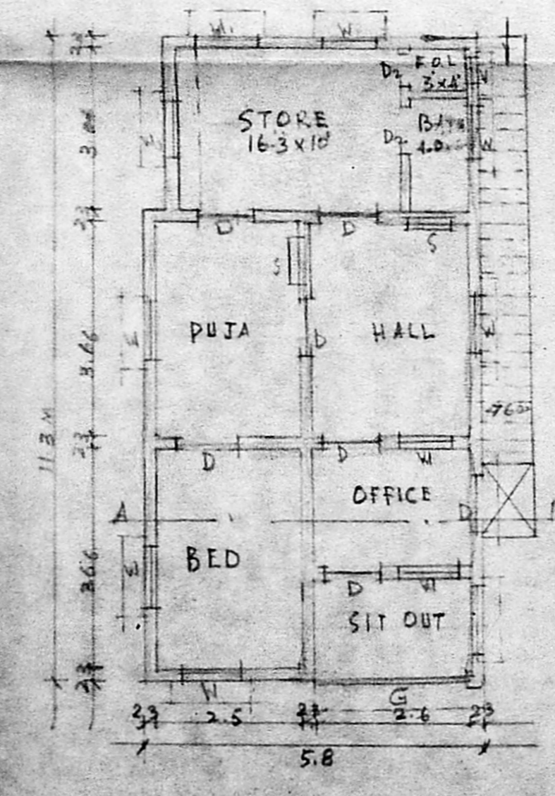
PRO. PLAN OF SECOND FLOOR
