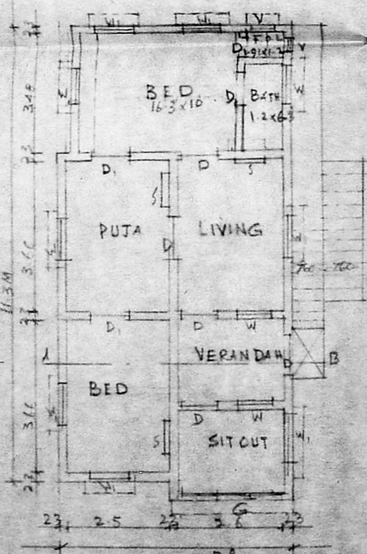
EXG. PLAN OF FIRST FLOOR
